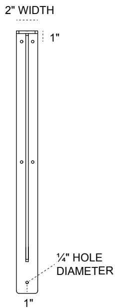
FRONT PROFILE
